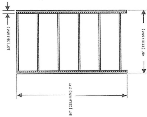
Modular Steel Shelving system SHORT LENGTH
